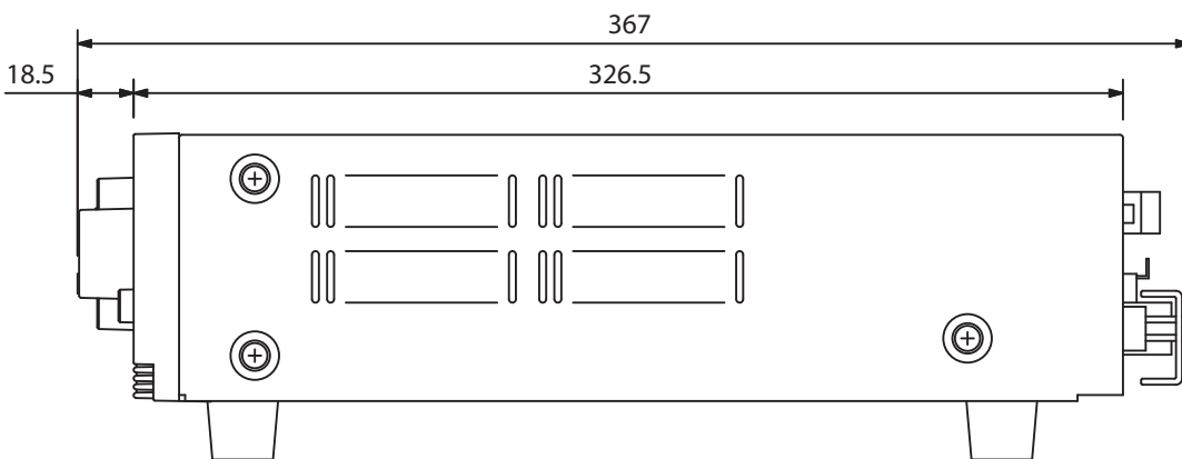
Side View
