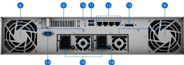
Rear (RS1221RP+)
