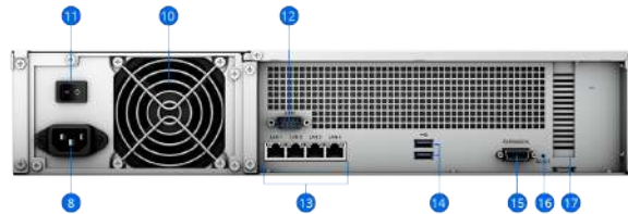
RS2421RP+ (Rear)
