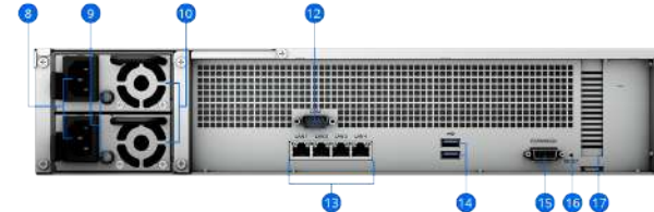
RS2421RP+ (Rear)
