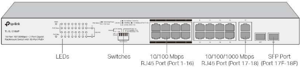
Figure 1-2 Front Panel of TL-SL1218MP
