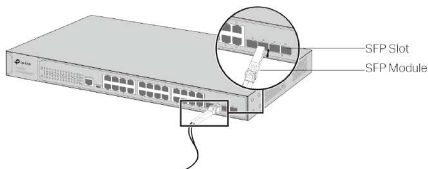
Figure 3-2 Inserting the SFP Module
