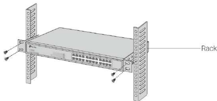
Figure 2-3 Rack Installation
