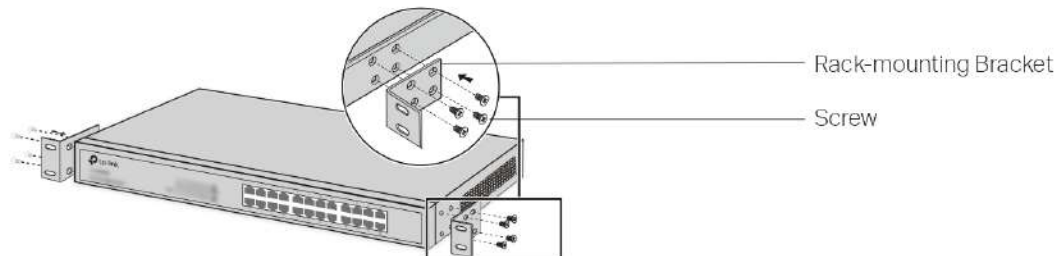
Figure 2-2 Bracket Installation
