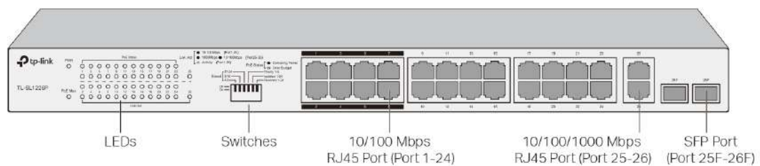
Figure 1-3 Front Panel of TL-SL1226P
