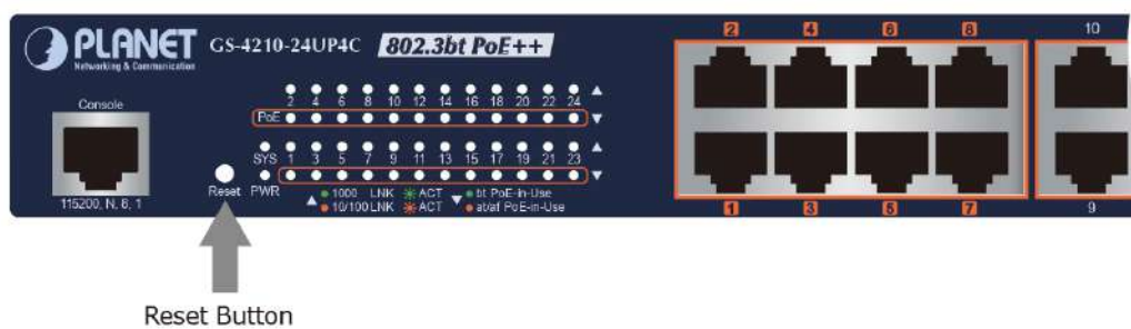
Figure 5-3: GS-4210-24UP4C Reset Button
