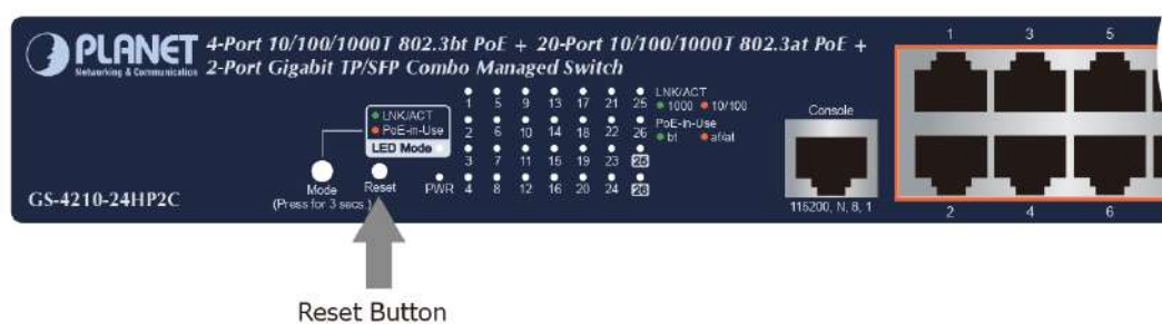
Figure 5-4: GS-4210-24HP2C Reset Button
