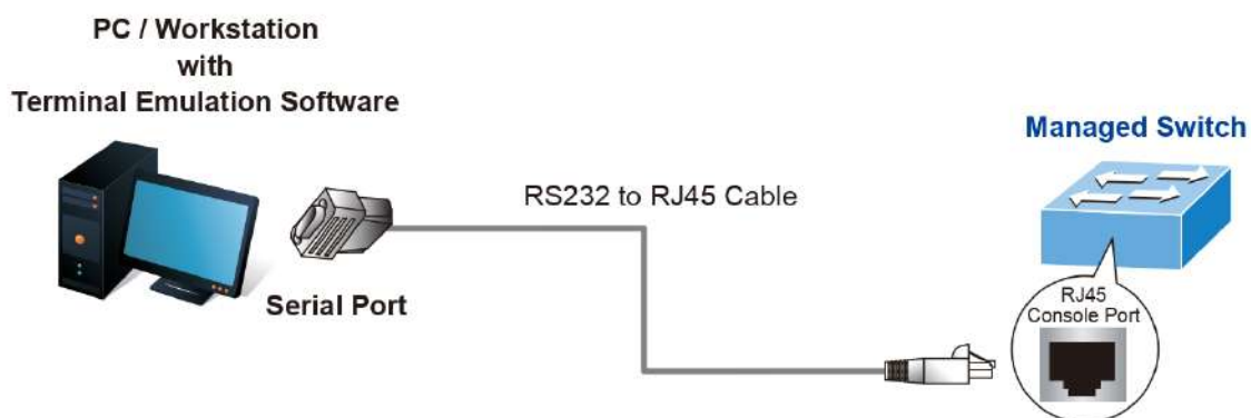
Figure 3-1: Managed Switch Console Connectivity
