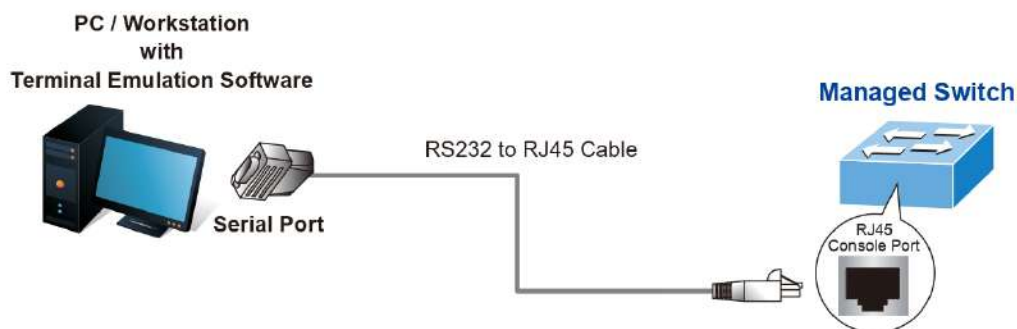
Figure 3-1: Managed Switch Console Connectivity
