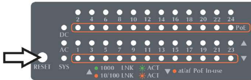
Figure 8-1: GS-5220-24P4X(R) Reset Button
