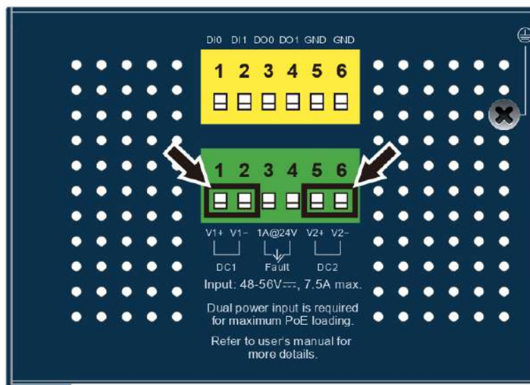
Figure 3-1: IGS-6325-16P4S Upper Panel
