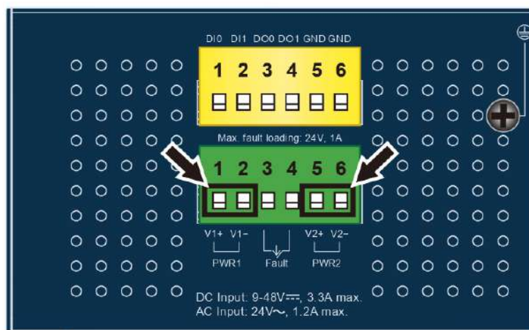
Figure 3-2: IGS-6325-16T4S Upper Panel
