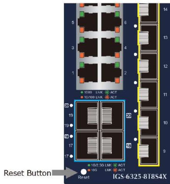
Figure 6-3: IGS-6325-8T4X/IGS-6325-8T8S/IGS-6325-8T8S4X Reset Button
