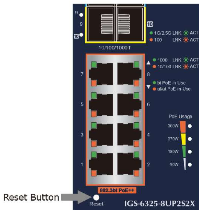
Figure 6-4: IGS-6325-8UP2S/IGS-6325-8UP2S2X Reset Button
