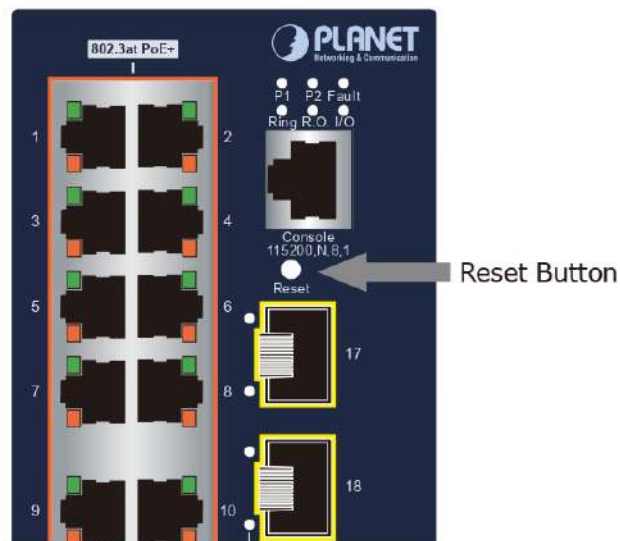
Figure 6-1: IGS-6325-16P4S/IGS-6325-16T4X Reset Button
