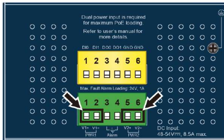
Figure 3-5: IGS-6325-8UP2S/IGS-6325-8UP2S2X Upper Panel
