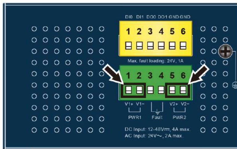
Figure 3-4: IGS-6325-8T4X/IGS-6325-8T8S/IGS-6325-8T8S4X Upper Panel
