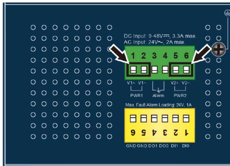
Figure 3-3: IGS-6325-16T4X Upper Panel
