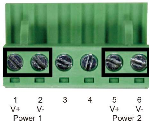
Figure 3-6: The pin of 6-contact terminal block connector
