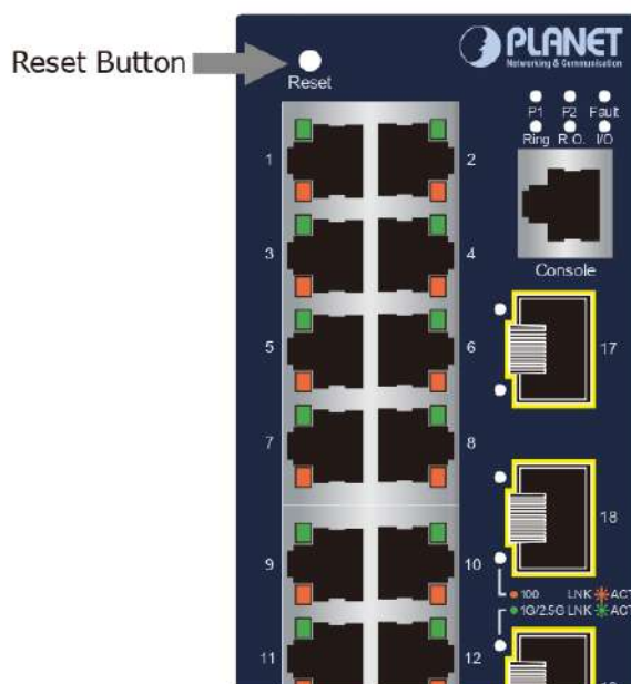
Figure 6-2: IGS-6325-16T4S Reset Button
