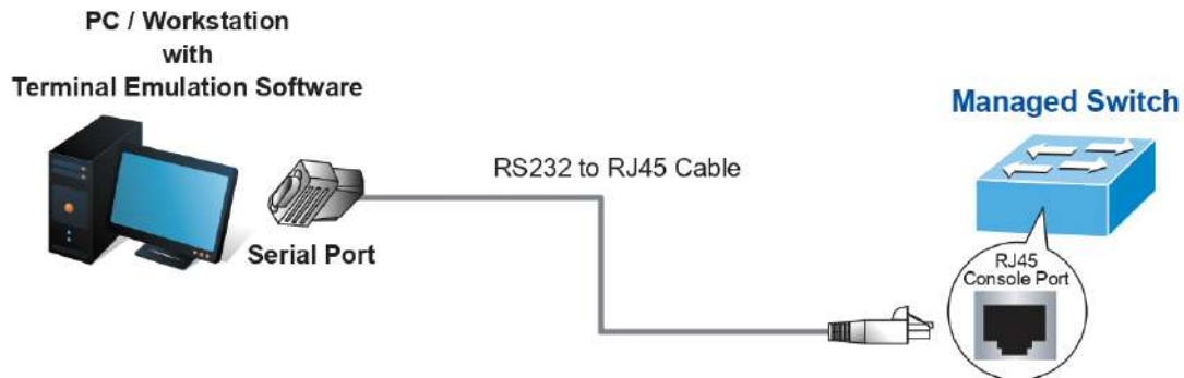
Figure 4-1: LRP Managed Switch Console Connectivity
