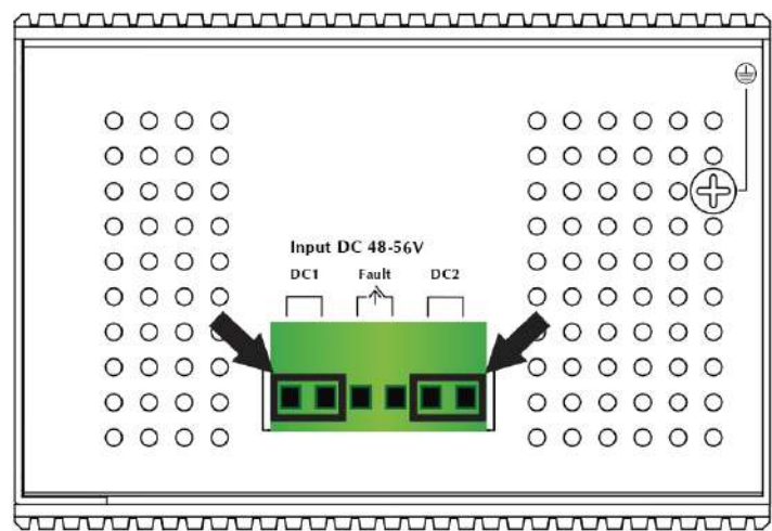
Figure 3-1: LRP-422CST Upper Panel
