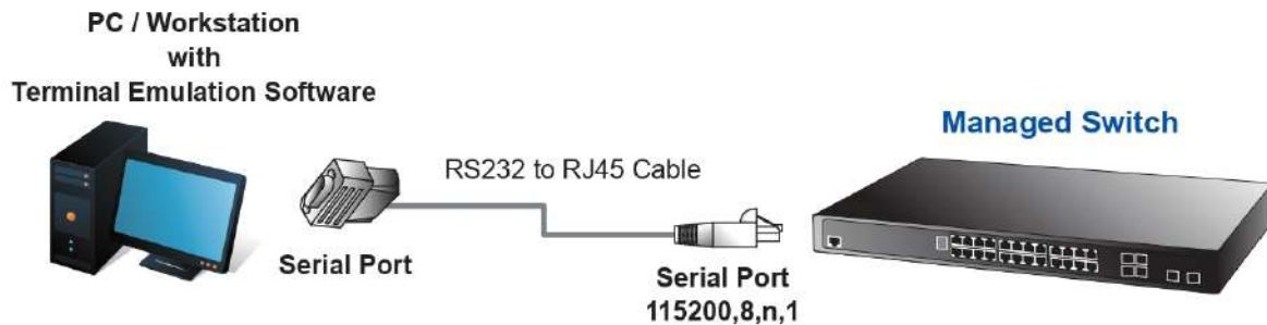
Figure 3-1 Stackable Managed Switch Console Connectivity
