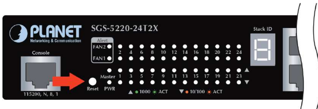
Figure 8-1: Stackable Managed Switch Reset Button
