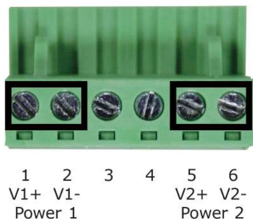
Figure 3-4: Power 1 & 2 Pins of Terminal Block Connector
