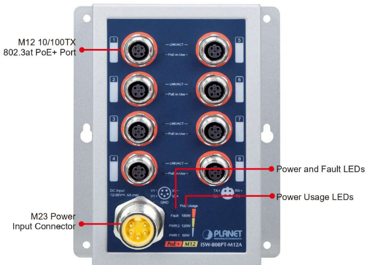
Figure 2-2: ISW-808PT-M12A Front Panel
