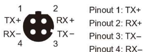
4-pin M12 Female 10/100TX Connector Pin Assignment
