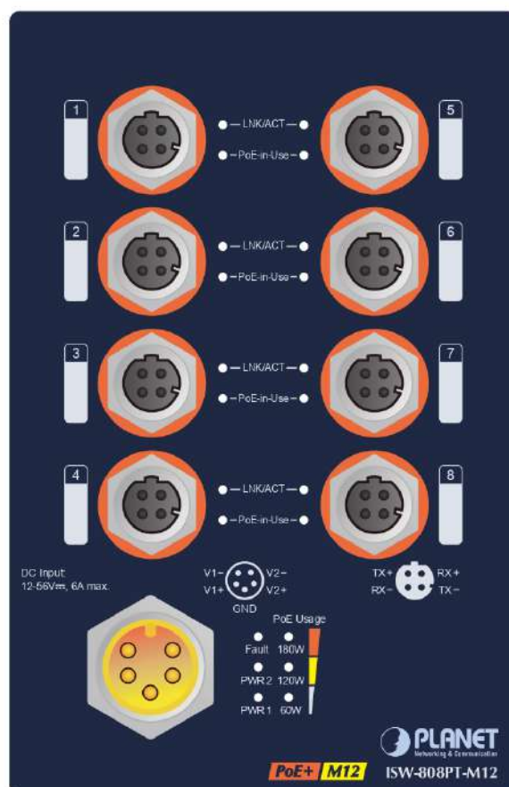
Figure 2-1: ISW-808PT-M12 Front Panel
